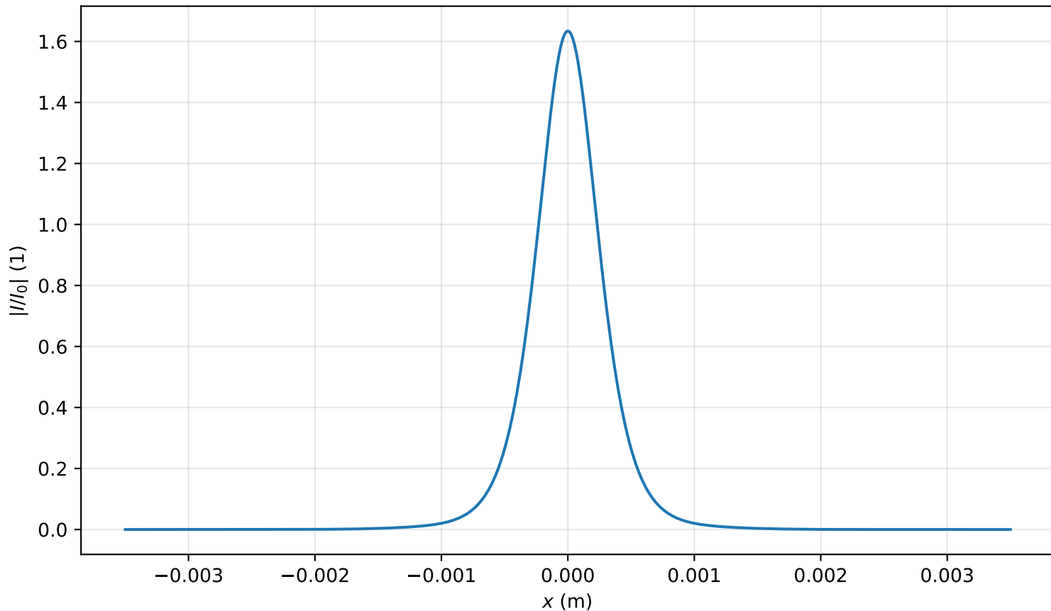
Intensity profile I(x, y = 0, z = 2.229m)/I_0 , P_{in}=0.9P_{cr} , artificial time
